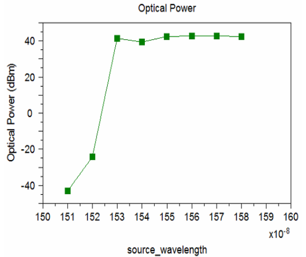
Fig. 6 (b) Fig. 9 Optical Power(dBm) v/s source wavelength (m) of EYCDFA
