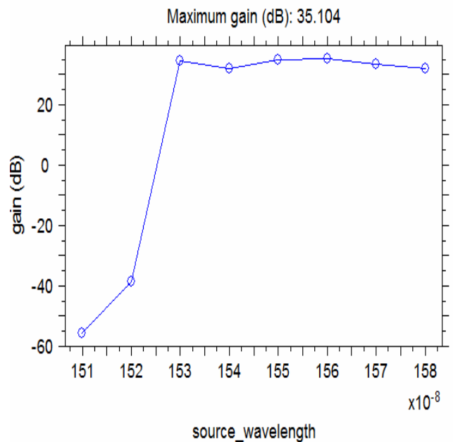
Fig.4 Gain(dB) v/s source wavelength(m) of EDFA
