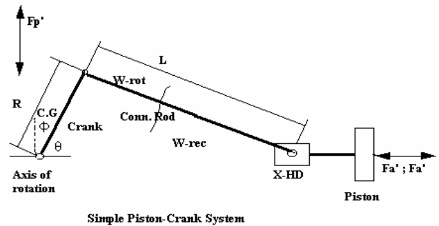
Fig 2: Simple piston crank system
