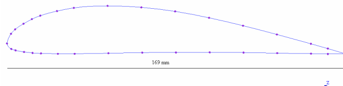
Fig: 2. The blade profile used in impeller is as shown above.
