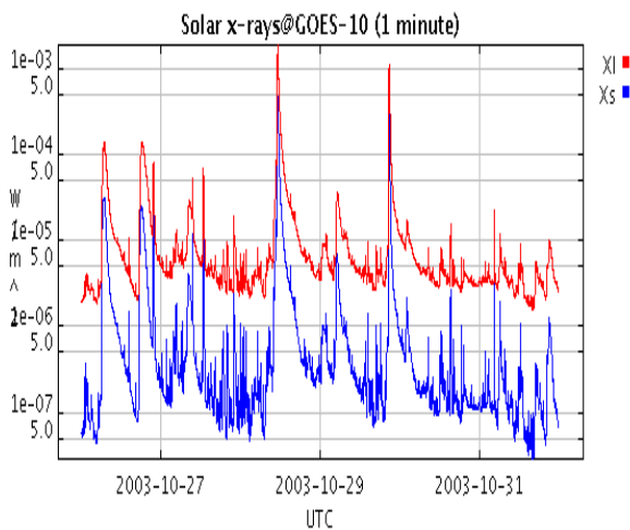
Here XL 1-8 Ang X-ray flux (watt/m 2 ) XS 0.5-3 Ang X-ray flux (watt/ m 2 )
