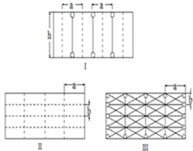
Fig. 3 Formulation of multiple strut
