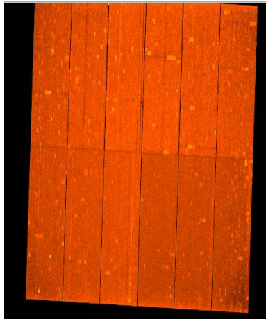
Fig. 6. (a) Image of a X-ray astronomical object
