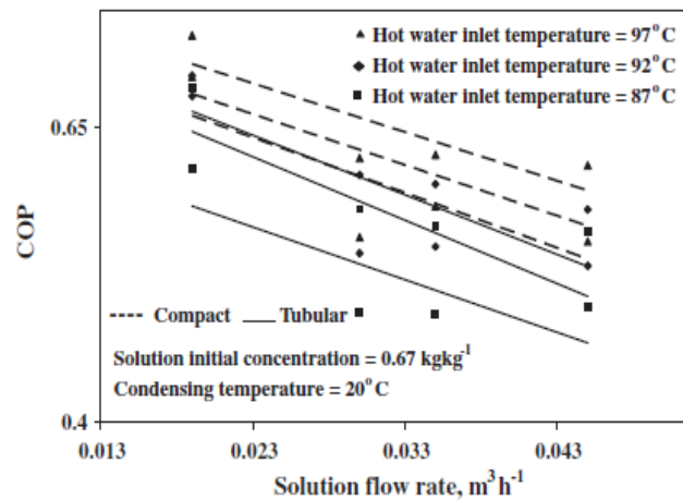
Fig. 9: Effect of solution flow rate on (a) circulation ratio and (b) COP for different hot water inlet temperatures [24].
