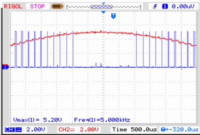
Fig. 7. Sine Triangle Comparison based PWM signal of 5 kHz with its reference sine wave
