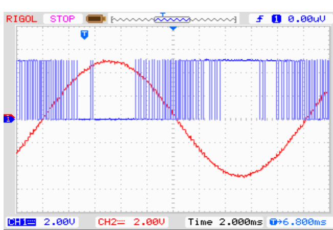
Fig. 6. 50 Hz reference sine wave and its corresponding PWM signal, generated using sine-triangle comparison technique at DSP board pin (40 - pin Berg-stick connector of DSP board)
