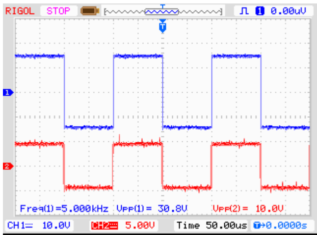
Fig. 2. Input and Output of GD card
