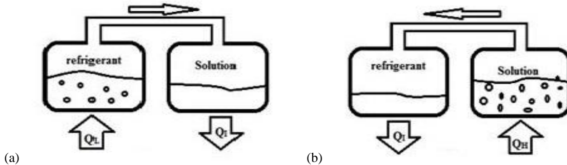
Fig. 1. (a) Absorption process occurs in right vessel causing cooling effect in the other; (b) Refrigerant separation process occurs in the right vessel as a result of additional heat from outside heat source.
