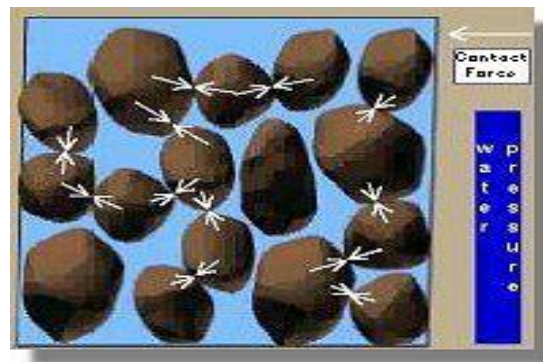
Fig.1. (c) The contact forces are small at high water pressure. In an extreme case, the pore water pressure may become so high that many of the soil particles lose contact with each other. (Reference: www.ce.washington.edu/~liquefaction )
