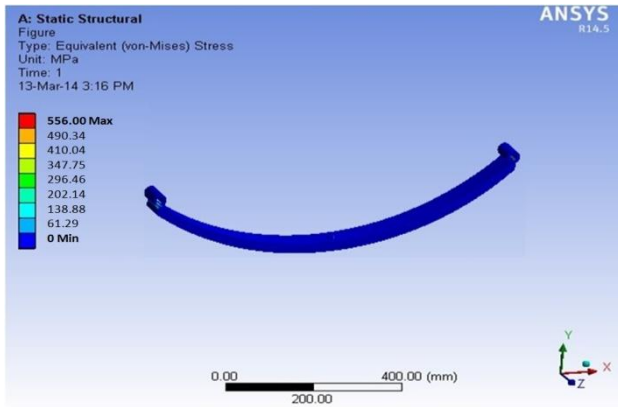
Figure 5.3 Stress generated on leaf spring
