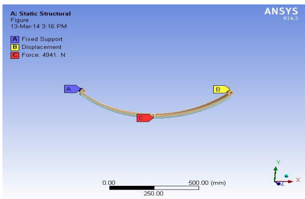
Figure 5.1 boundary condition for rectangular cross section
