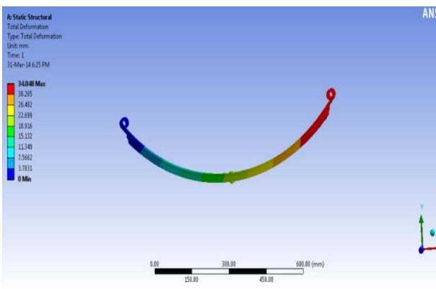
Figure 5.6 Deflection of leaf spring
