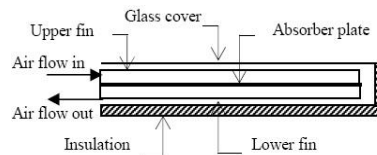
Fig.4. Schematic of the double pass solar collector with longitudinal fin [15]
