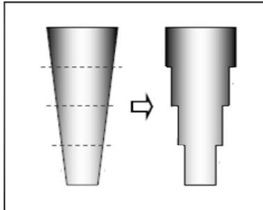
Fig.1 Actual taper pile and idealized taper pile
