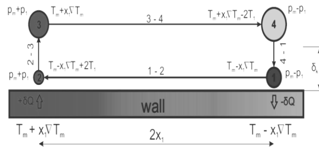
Fig. 1. The parcel of gas which is neither isothermal nor adiabatic has imperfect thermal contact with the wall (a macroscopic Lagrangian view)
