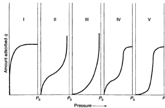
Fig.2.The five types of Isotherms (Courtesy: Adsorption Technology and Design, Thomson and Crittenden, Butterworth)
