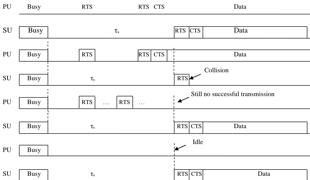
Fig. 3 CSMA based protocols with four-way handshaking procedure coexists with the PS. [3]
