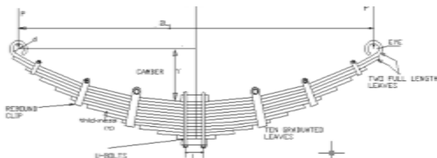
Figure 1.1 semielliptical leaf spring
