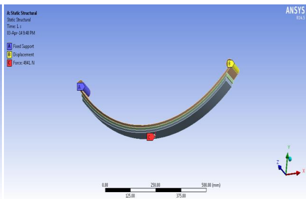
Figure 5.2 boundary condition for trapezoidal cross section
