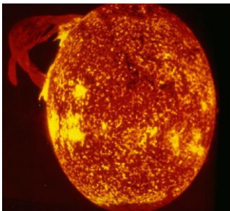
Fig. 1. Sun with a solar flare [2] After a solar flare [9]
