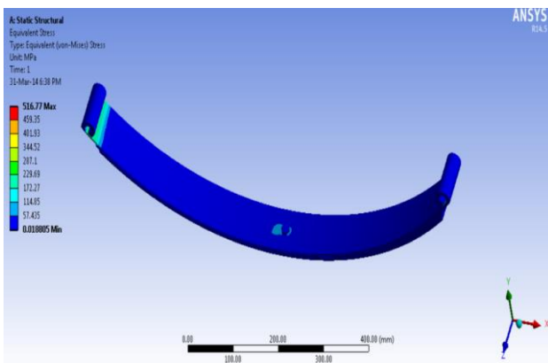
Figure 5.5 Stress generated on leaf spring
