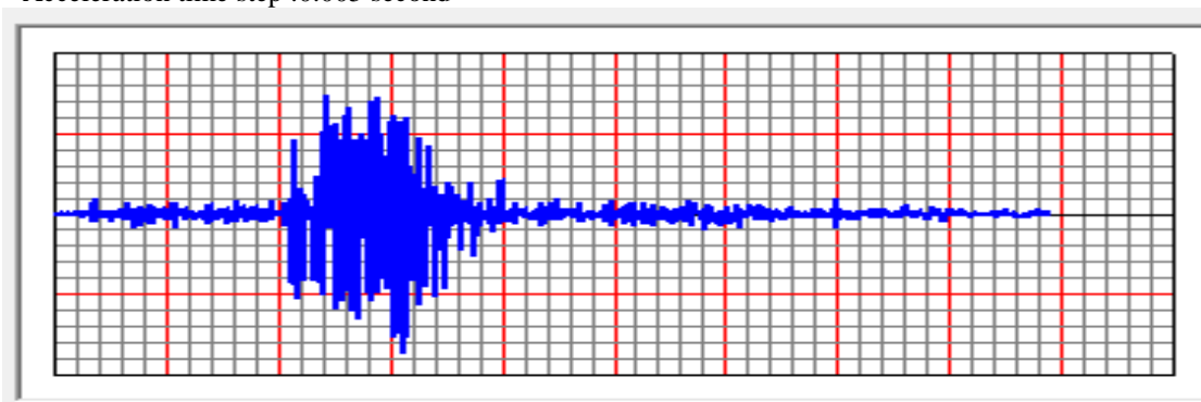
Fig. 3 Bhuj Acceleration time History
