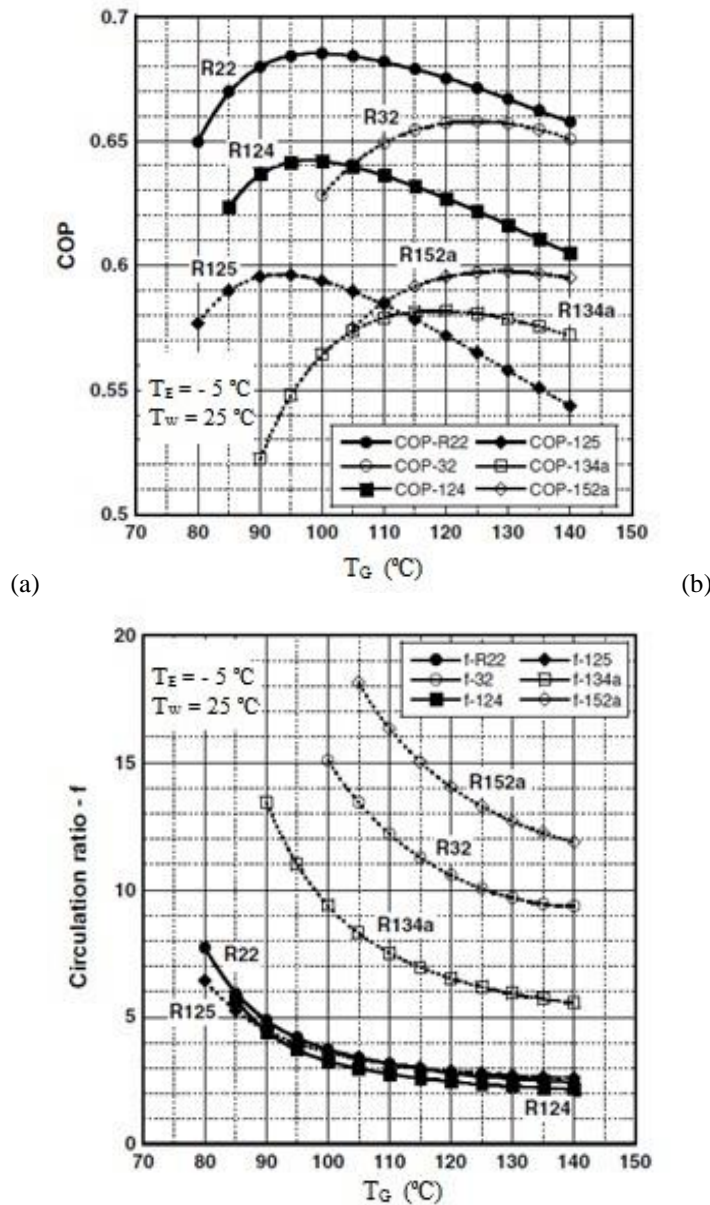
Fig. 8. Variation of (a) COP and (b) circulation ratio with generator temperature, for evaporator temperature of -5°C and cooling water temperature of 25°C [17].
