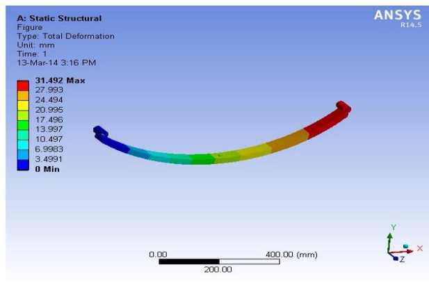
Figure 5.4 Deflection of leaf spring
