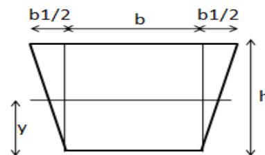
Figure 4.2 trapezoidal cross section of leaf spring
