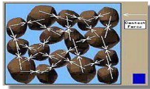
Fig.1. (b) The length of the arrows represents the size of the contact forces between individual soil grains. The contact forces are large when the pore water pressure is low.
