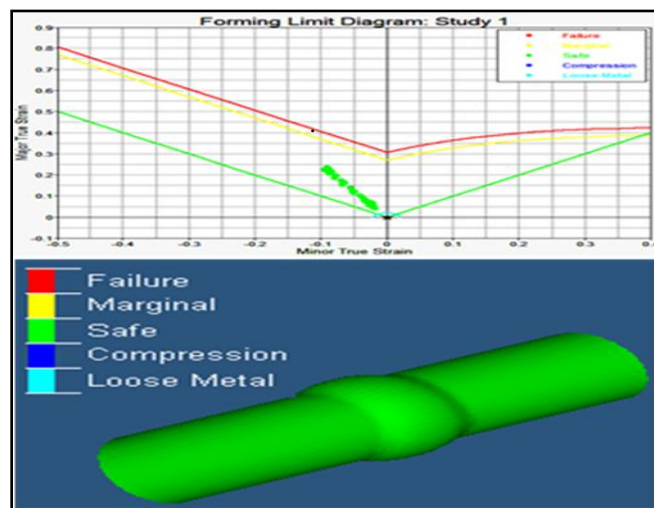
Fig.16 FLC &amp; FLD Curve
