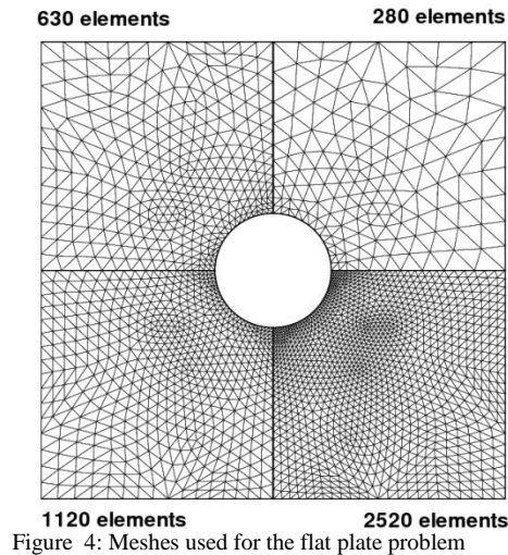
Figure 4: Meshes used for the flat plate problem
