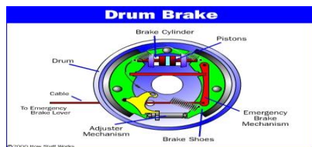
Figure 4.3 Drum brake
