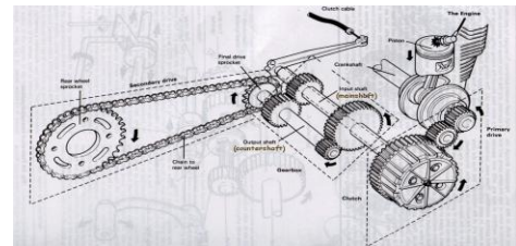
Figure 4.7 Motorcycle drive train systems
