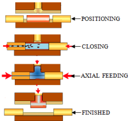
Fig. 1 Hydroforming Sequences for T-Shape
