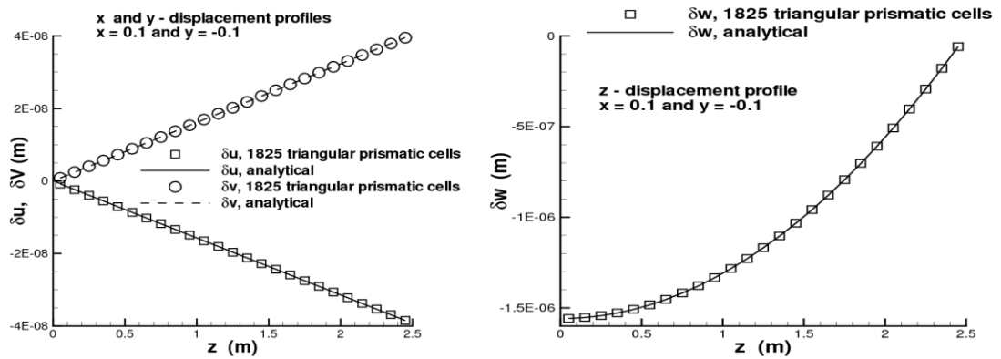
(a) x and y - displacements, x = 0.1 m and y = -0.1 m (b) z - displacement, x = 0.1 m and y = -0.1 m
