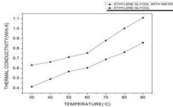
Fig.7. Measured thermal conductivity of \text{Al}_2\text{O}_3 -EG- \text{H}_2\text{O} and \text{Al}_2\text{O}_3 -EG nanofluid.
