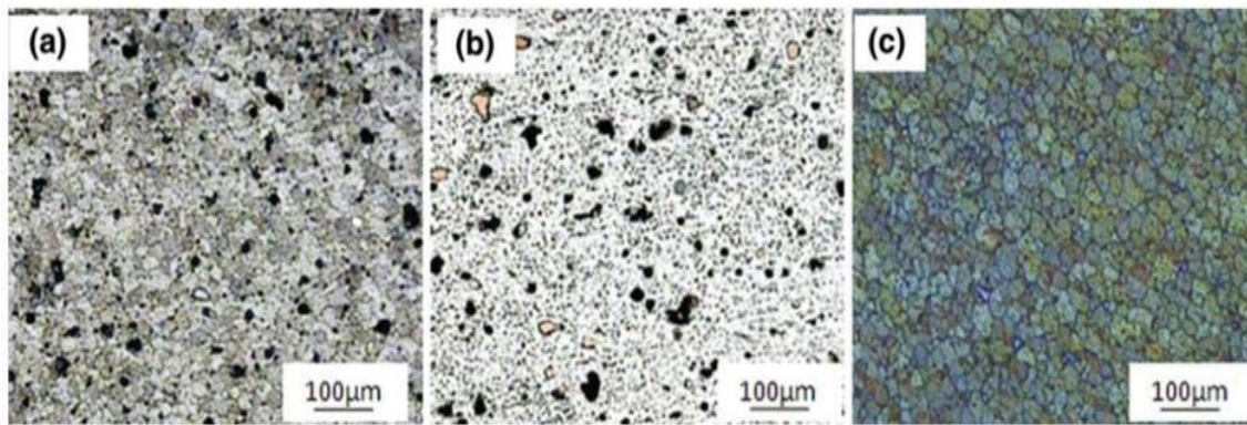
Fig. 6. Microstructures of Al 2024 – O with different reagent a Keller's etch b week's etch c new technique [31]
