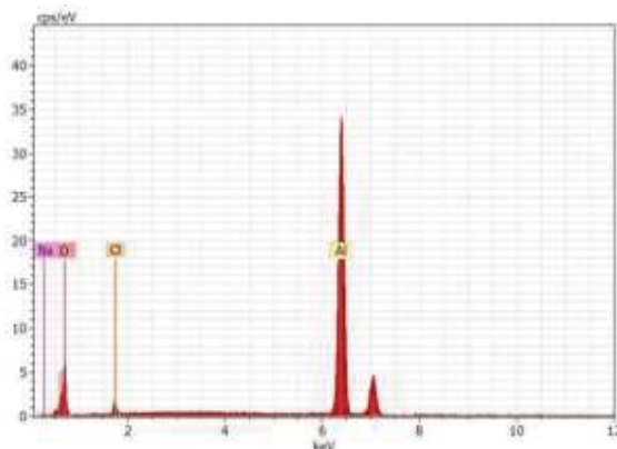
Fig.3 Chemical composition of synthesis \text{Al}_2\text{O}_3 nanoparticles using EDS
