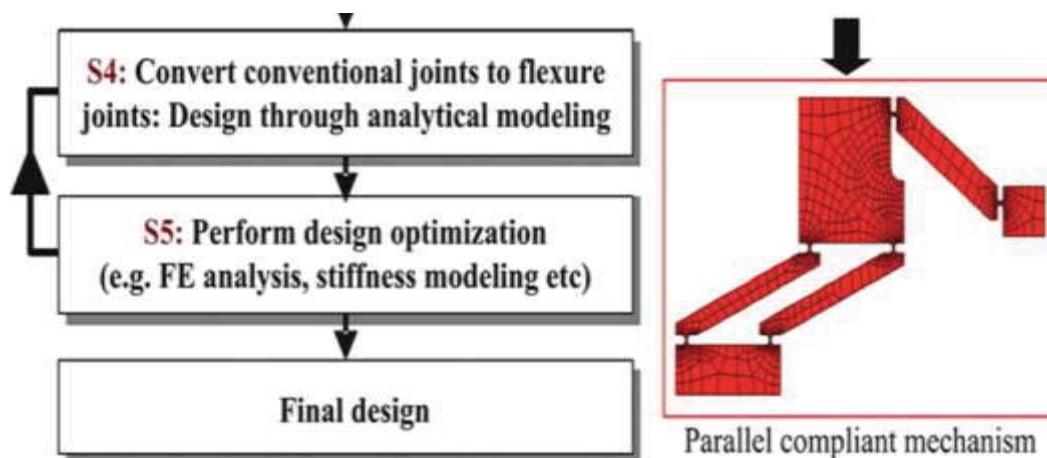
Fig. 5 Linkage-joint made up of parallel-kinematic architecture and parallel compliant mechanism [23]
