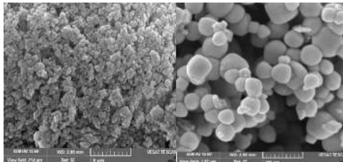
Fig. 2 Surface morphology of the \text{Al}_2\text{O}_3 nanoparticles with respect to two different magnifications
