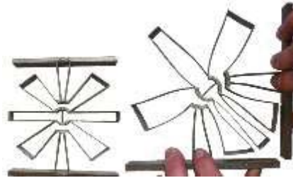
Fig. 4 A Complaint titanium hinge made with EBM. It has efficient of -90° to +90° of movement [12].
