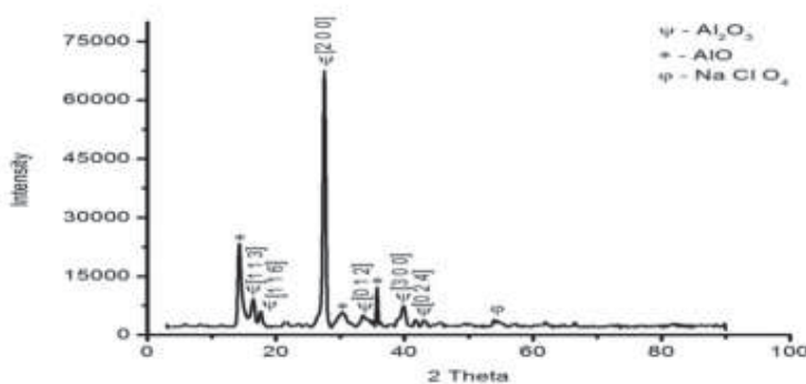
Fig.4. XRD pattern of \text{Al}_2\text{O}_3 Nanoparticle
